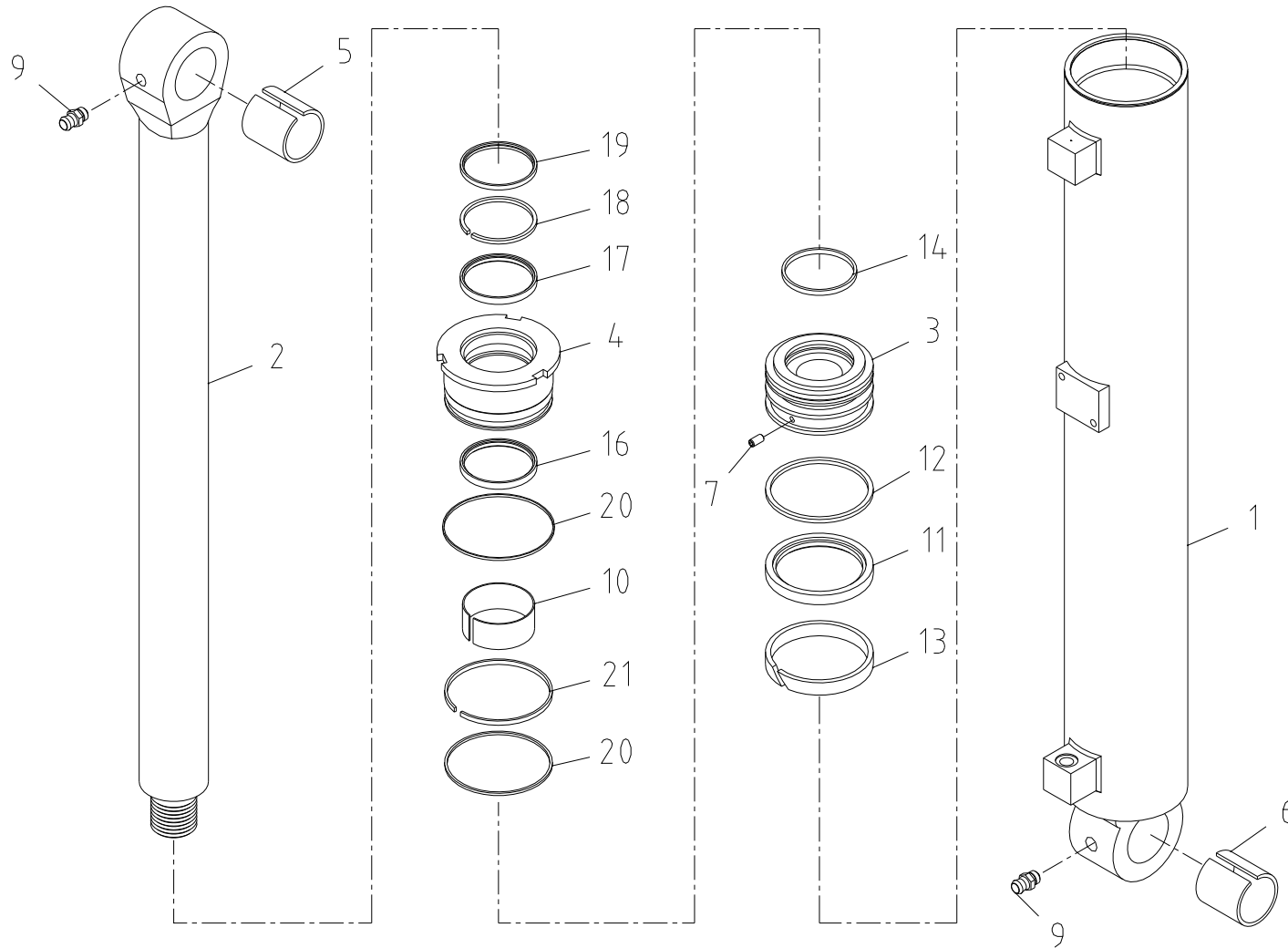
Fig. 2-1 SCS1015 DERRICK CYL' ASS'Y
