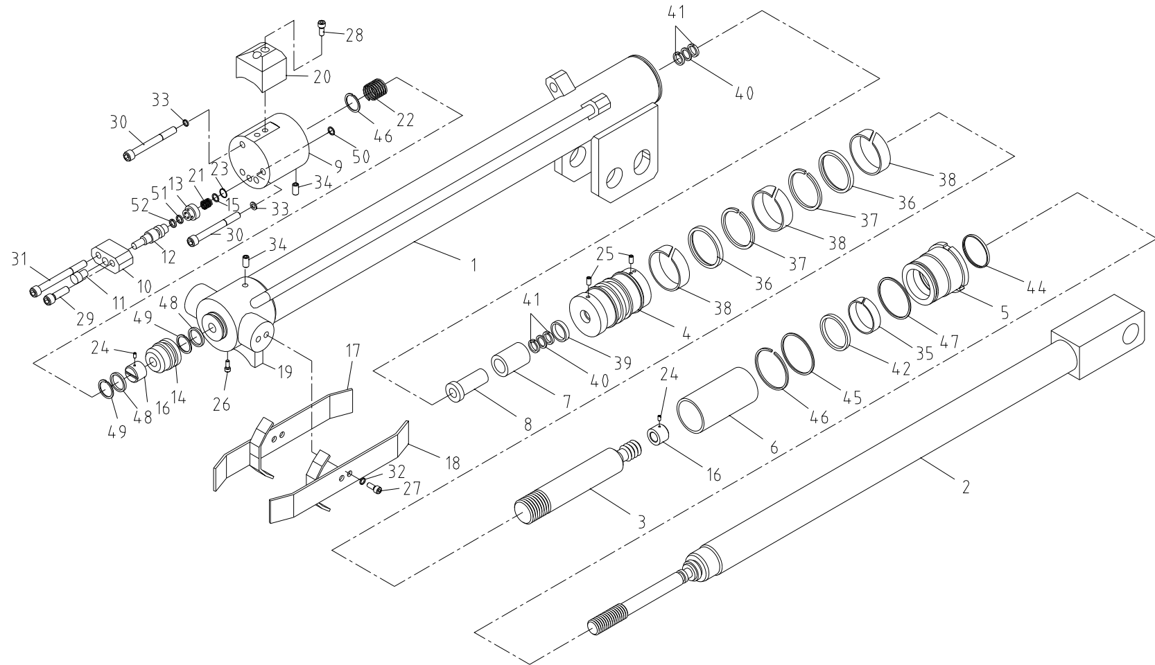
Fig. 1-1-1 SCS1015 TELESCOPIC CYL'(1st) ASS'Y
