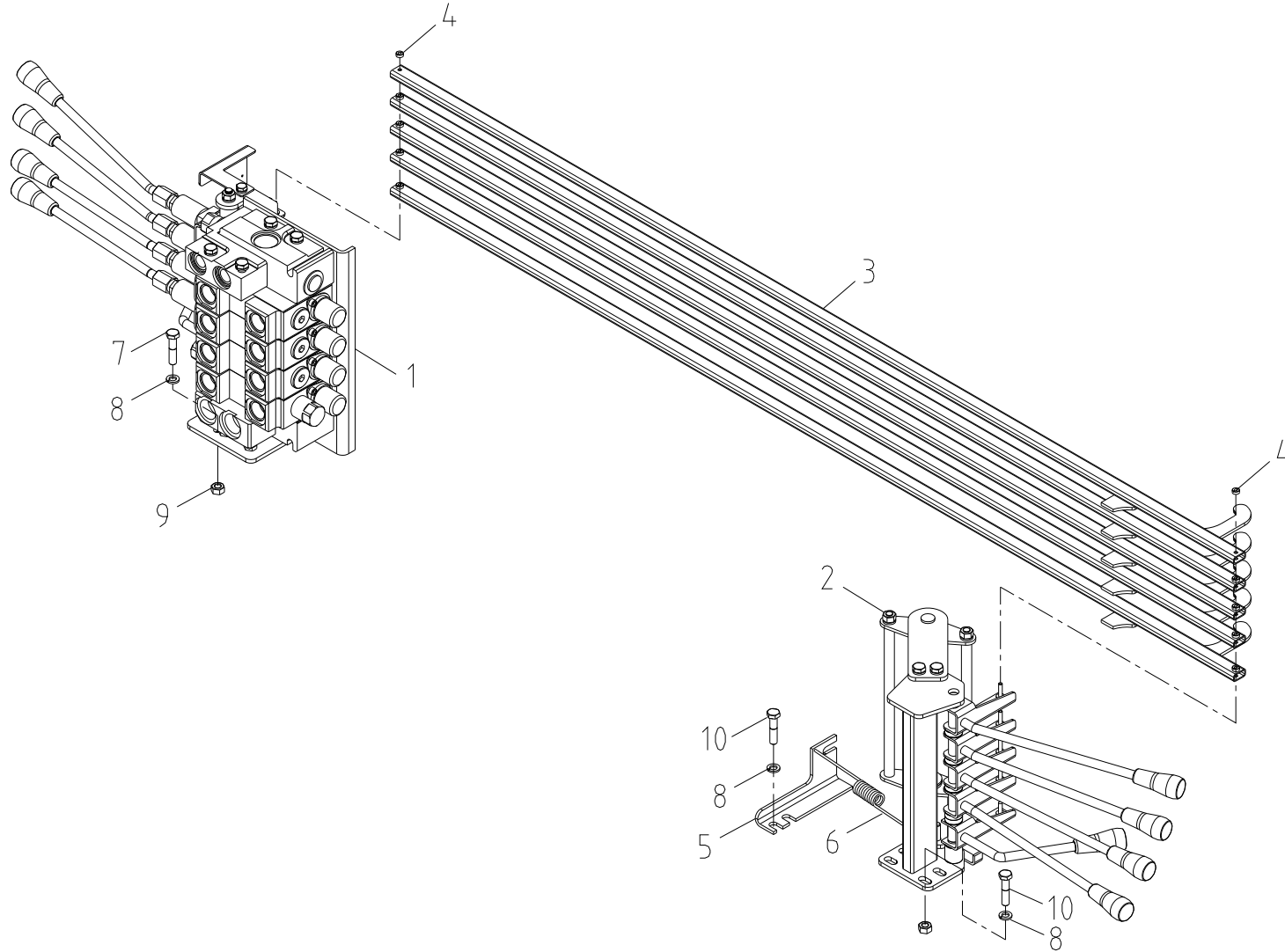
Fig. 3-3 SCS1015 OPERATION ASS'Y (1)
