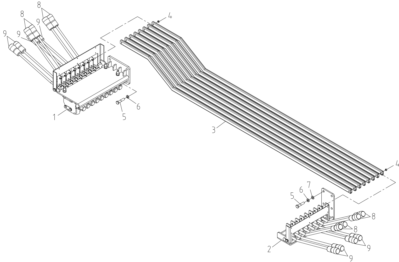
Fig. 3-4 SCS1015 OPERATION ASS'Y (2)
