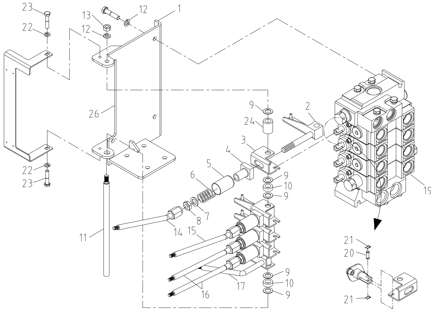
Fig. 3-3-1 SCS1015 VALVE STAND SET
