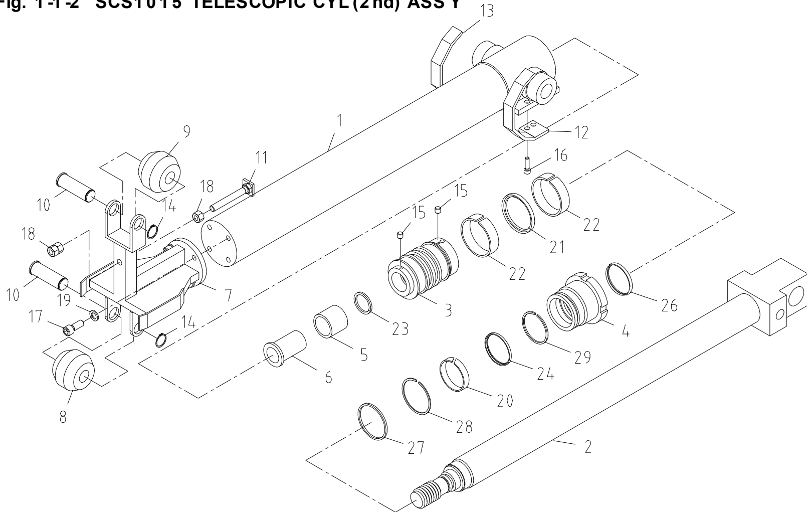
Fig. 1-1-2 SCS1015 TELESCOPIC CYL'(2nd) ASS'Y
