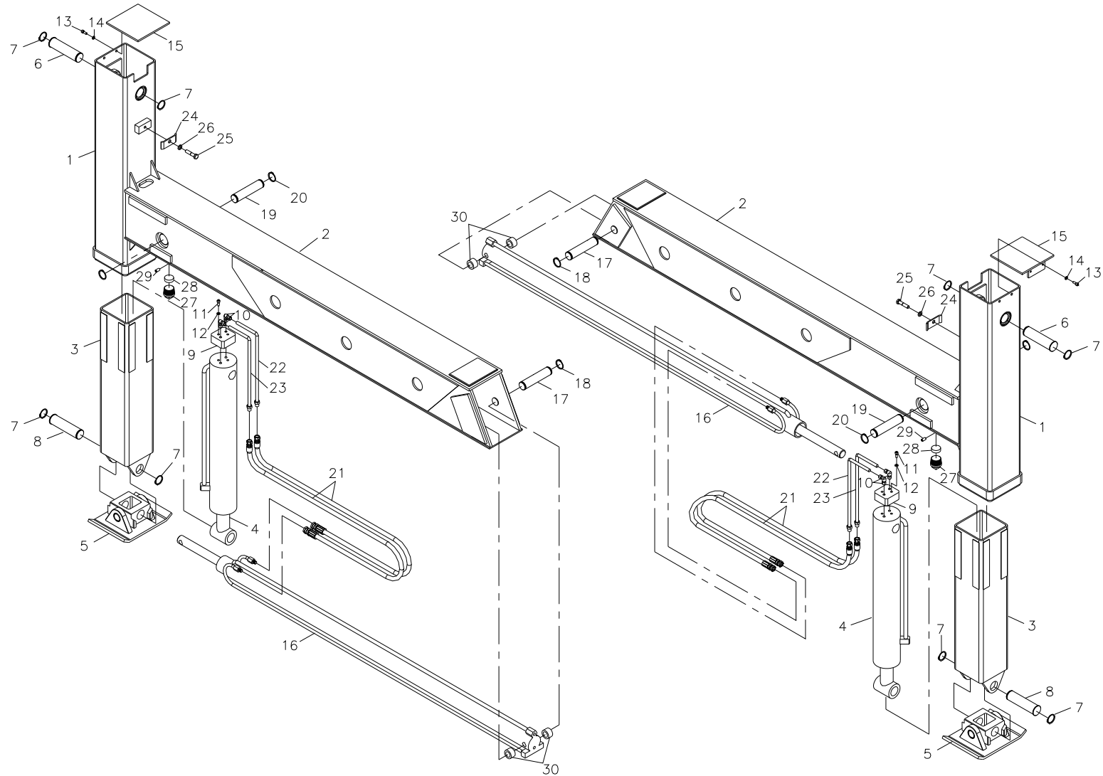
Fig. 8-2-1 SCS1015 REAR OUTRIGGER ASS'Y
